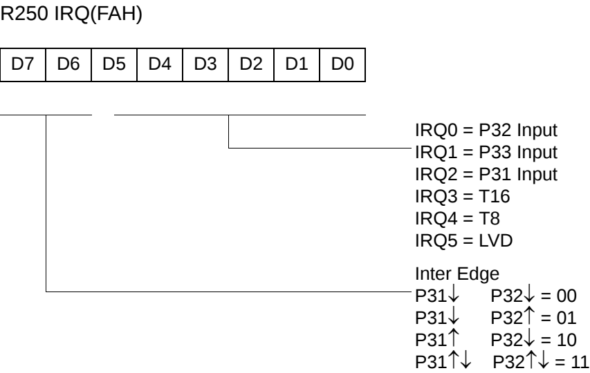
Figure 52. Interrupt Request Register (FAH: Read/Write)
