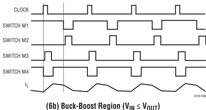
Figure 6. Buck-Boost Region
