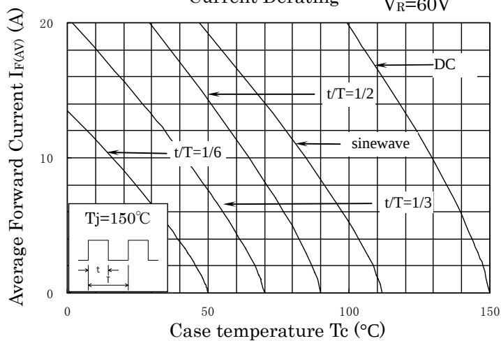
Current Derating
