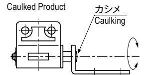
カシメ品 Caulked Product
