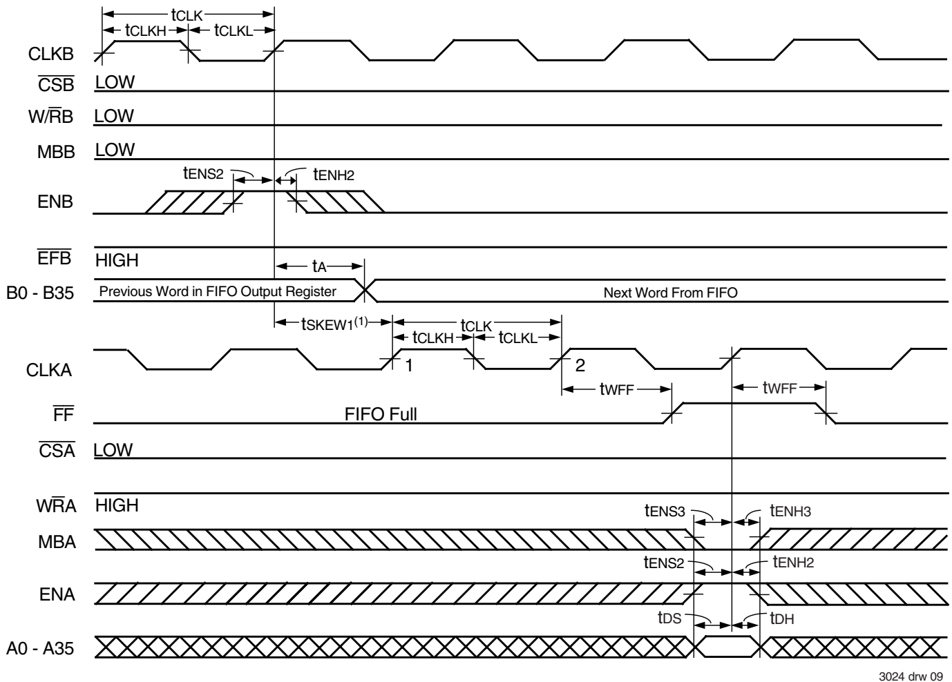
Figure 6. \overline{FF} Flag Timing and First Available Write when the FIFO is Full
