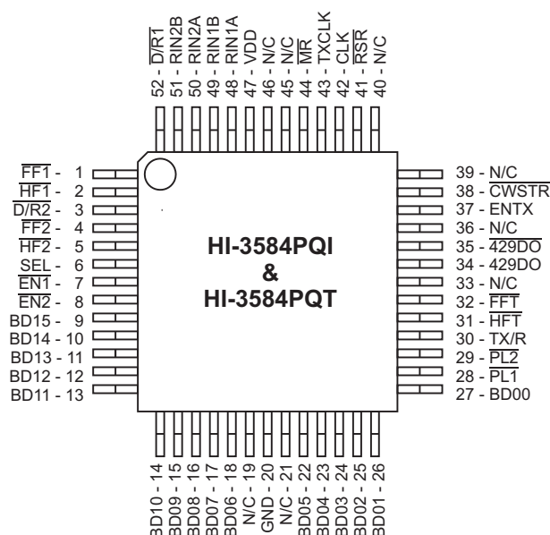
52 - Pin Plastic Quad Flat Pack (PQFP)
