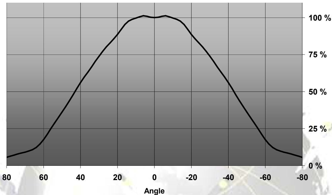
Relative Intensity of Flare-C-DIFF (vertical)
