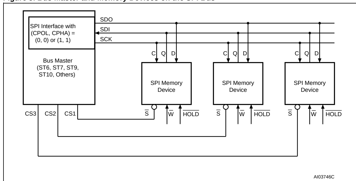
Figure 3. Bus Master and Memory Devices on the SPI Bus
