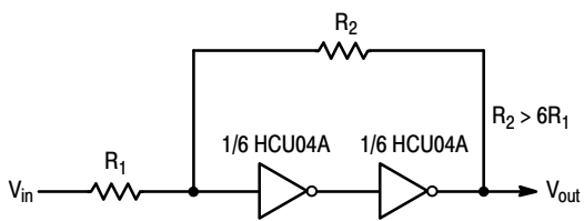
Figure 7. Schmitt Trigger
