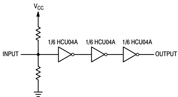
Figure 9. Multi-Stage Amplifier
