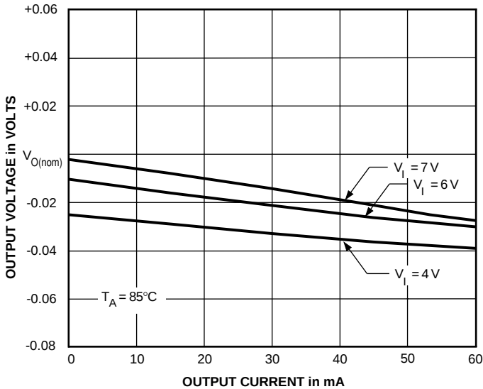
LOAD REGULATION
