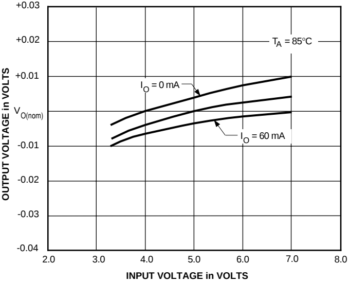
LINE REGULATION
