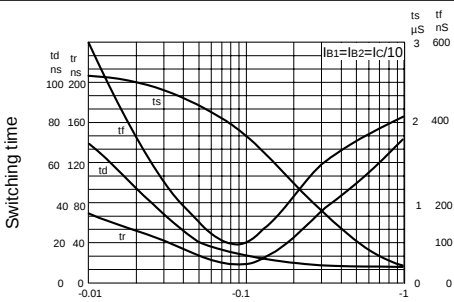
Switching Speeds
