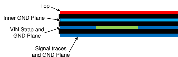
Figure 10-2. Example Layout for VQFN Package
