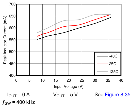
Figure 6-6. I_{PEAK-MIN}
