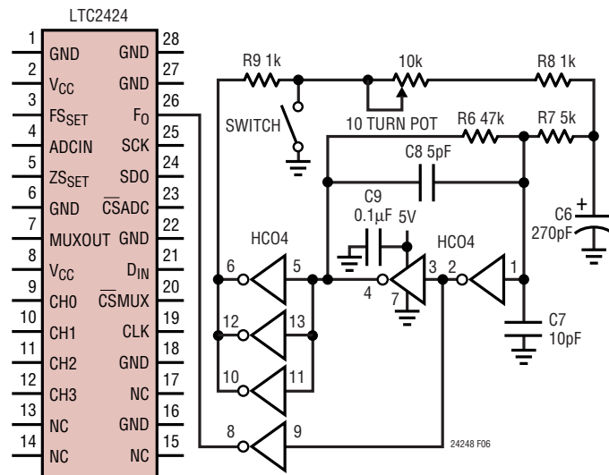
Figure 6. Selectable 100 Sample/Second Turbo Mode
