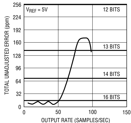
Figure 7. Total Error vs Output Rate ( V_{\text{REF}} = 5\text{V} )
