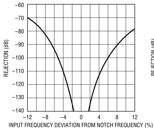
Rejection vs Frequency at V_{\text{IN}}
