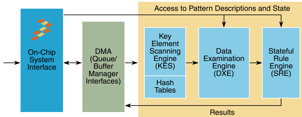
Figure 7. PME 2.1 Block Diagram
