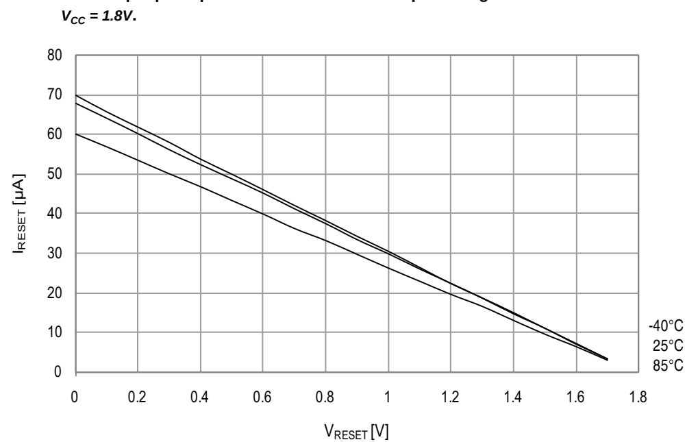
Figure 34-118. Reset pin pull-up resistor current vs. reset pin voltage.
