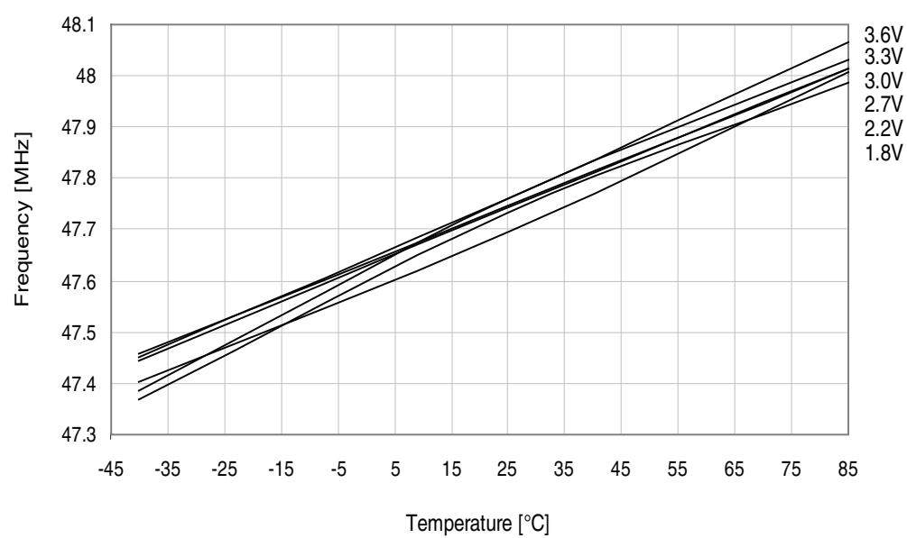
Figure 34-267.48MHz internal oscillator frequency vs. temperature. DPLL enabled, from the 32.768kHz internal oscillator.
