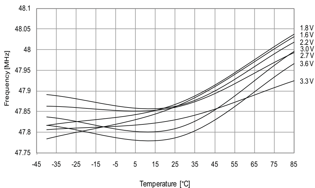
Figure 34-65. 48MHz internal oscillator frequency vs. temperature. DPLL enabled, from the 32.768kHz internal oscillator.
