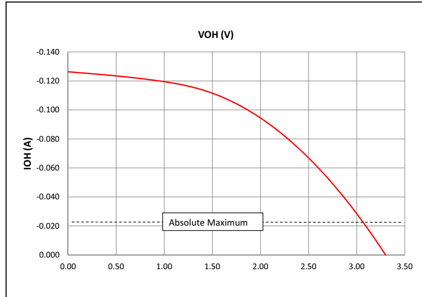
FIGURE 37-5: V_{OH} – 12x DRIVER PINS
