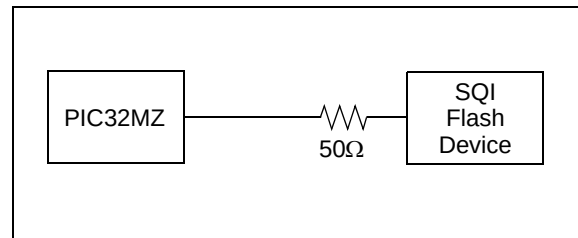
FIGURE 2-4: SERIES RESISTOR
