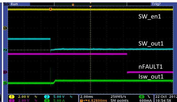
Figure 41. USB Switch1 Current Limit Operation
