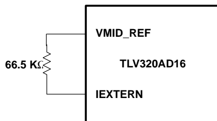
Figure 16. Bias Current Provided By On-Chip Voltage Reference
