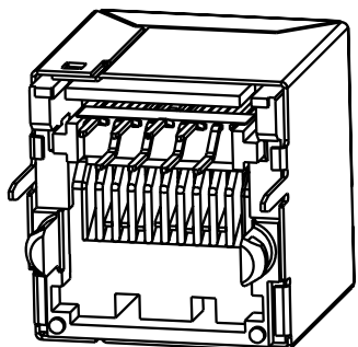
ISO VIEW
