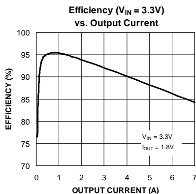
Figure 2. Efficiency Curve
