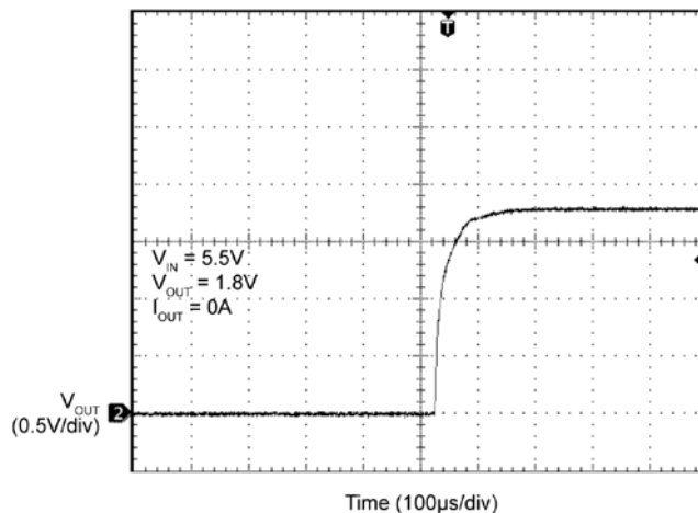
Switching Waveforms
