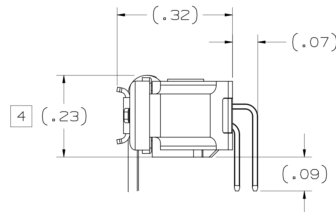
RA ASSEMBLY
