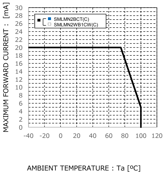
Fig.4 Derating
