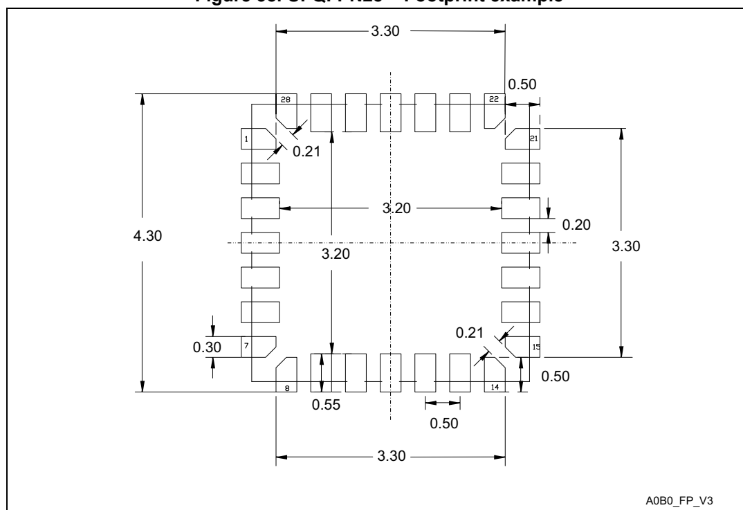
Figure 38. UFQFPN28 – Footprint example
