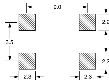
Figure 3) Land Pattern
