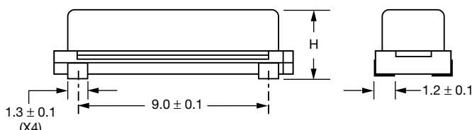
Figure 1) CSM-4AX- Top, Side and End views
