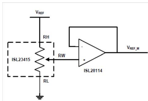
FIGURE 2. V_{\text{REF}} ADJUSTMENT
