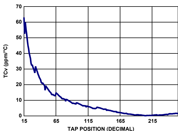
FIGURE 14. 50k TCv vs TAP POSITION
