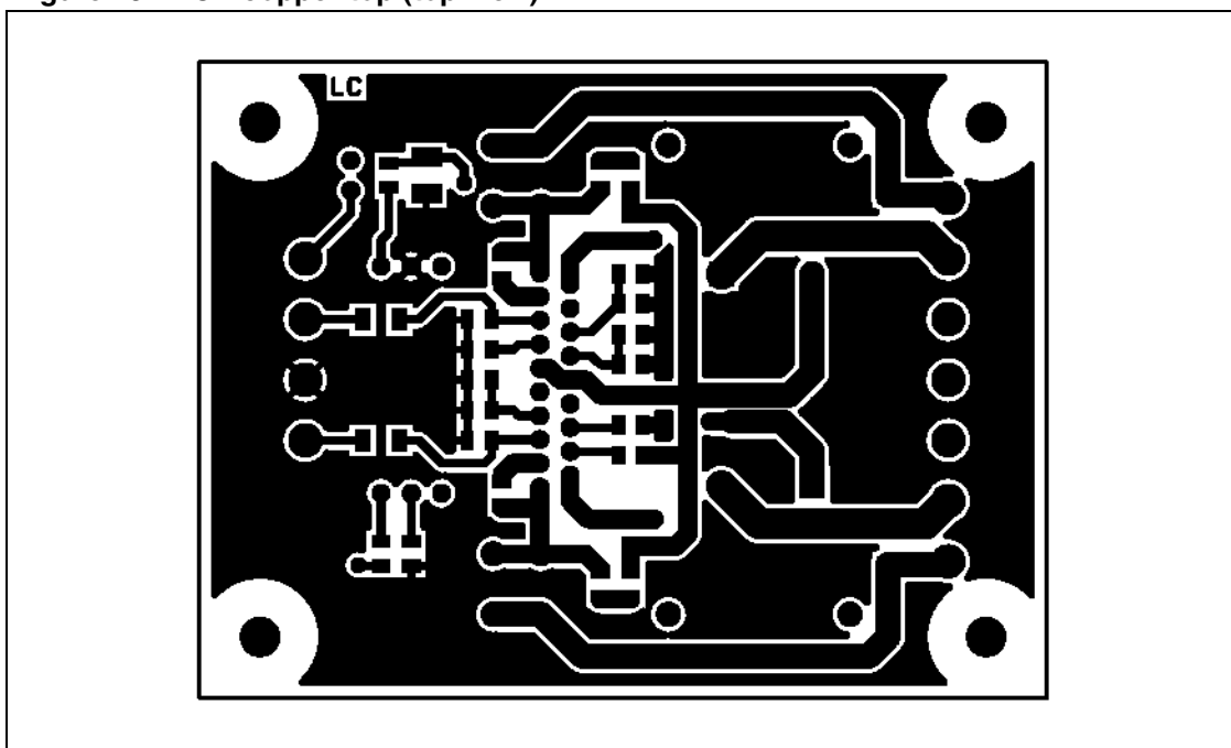
Figure 13. PCB copper top (top view)
