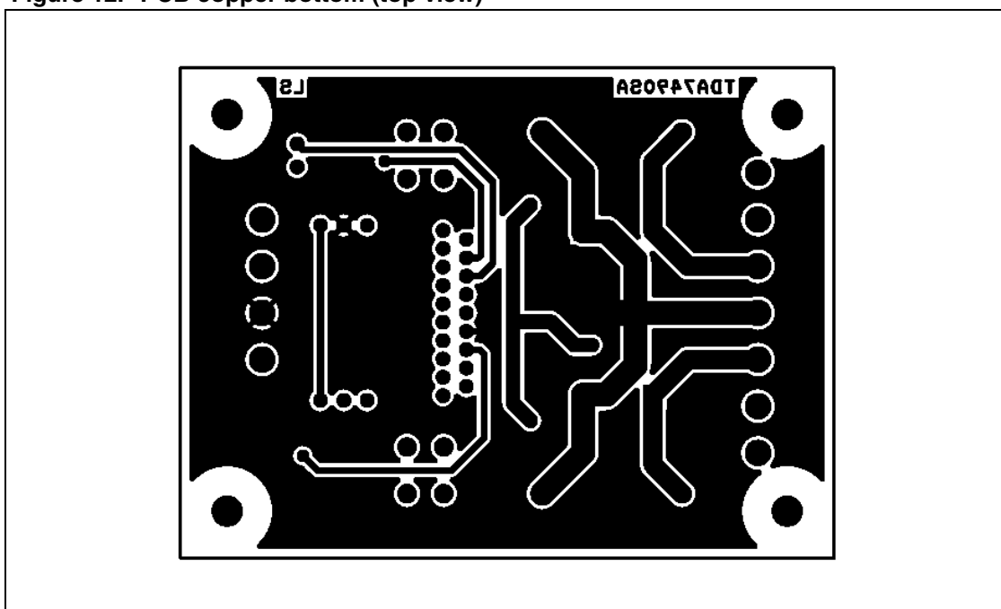
Figure 12. PCB copper bottom (top view)
