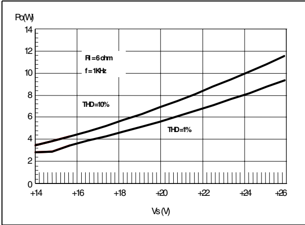
Figure 7. output power vs supply voltage (single)
