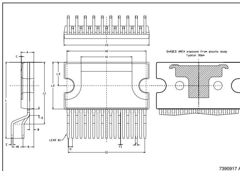
Clipwatt19
