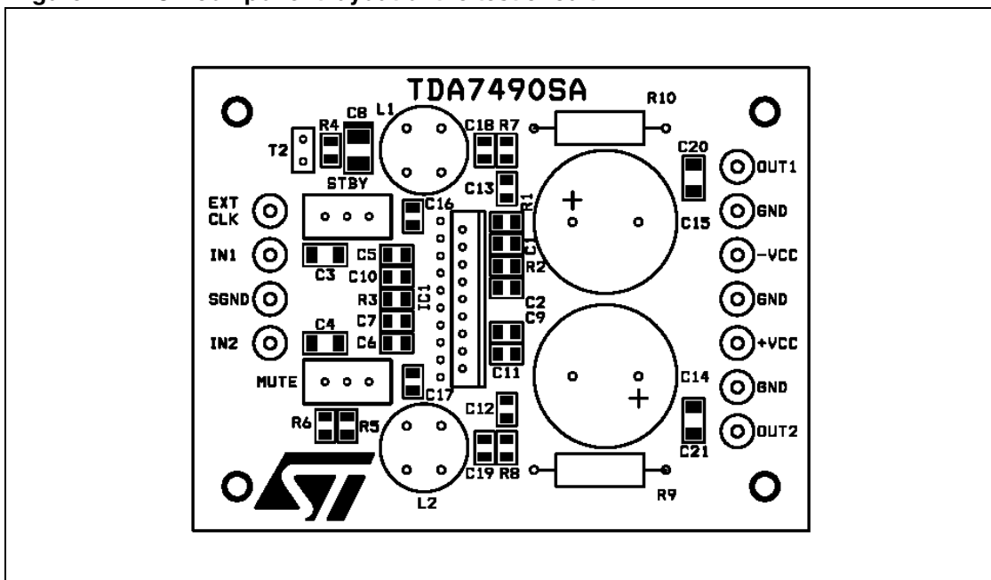
Figure 11. PCB component layout of the test circuit
