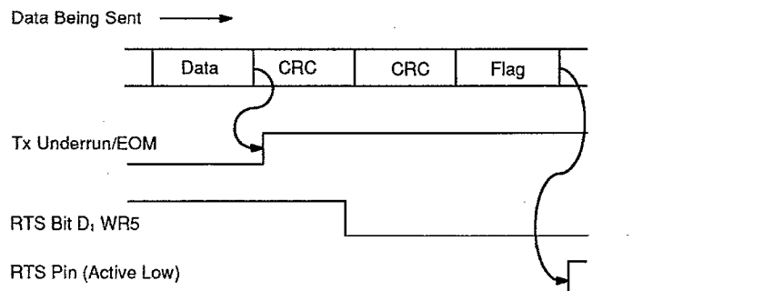
Figure 16. Auto \overline{\text{RTS}} Reset Mode
