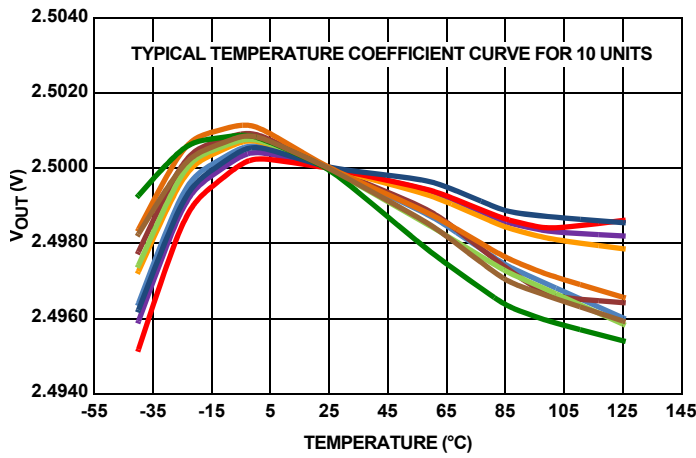
FIGURE 84. V_{OUT} vs TEMPERATURE
