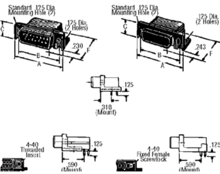
.318 Mount, .125" PC Board Posts
