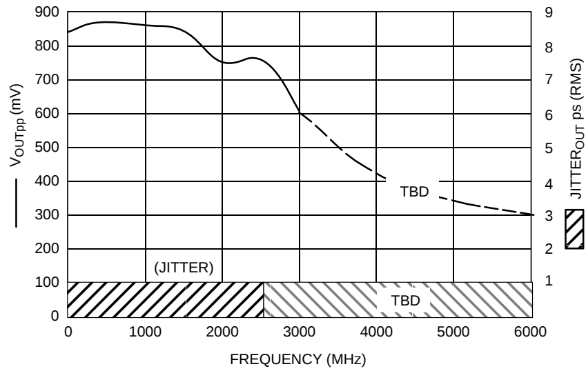
Figure 2. F_{\max}/\text{Jitter}
