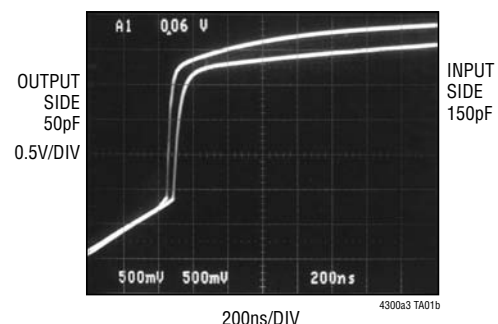
Input-Output Connection
