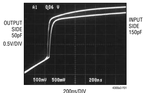
Figure 1. Input-Output Connection Low to High Transition
