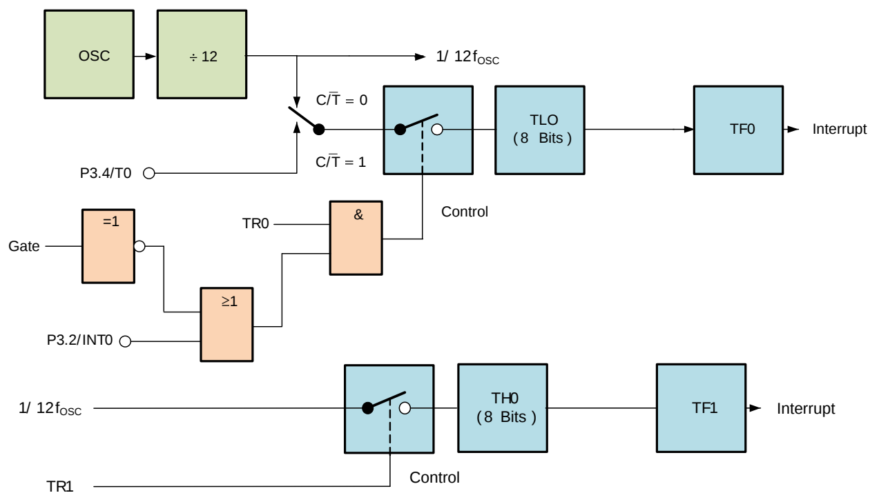
Figure 10. Timer 0 Mode 3
