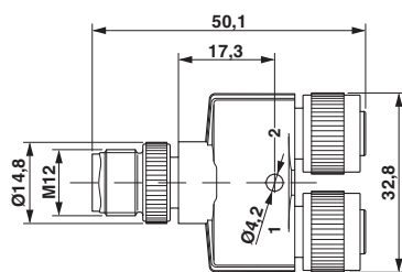
Dimensioned drawing
