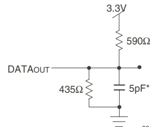
Figure 2. Output Test Load *Including scope and jig. (For tLZ, tHZ, twz, tow)
