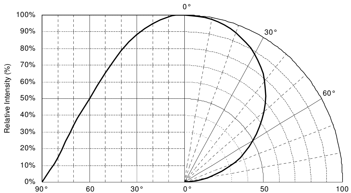
Fig 2. Radiation Characteristics
