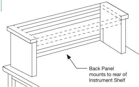
Upper Bin Holding Panel Illustrated
