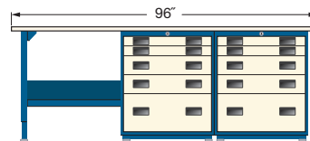
2 Cabinets + 1 Leg Assembly
