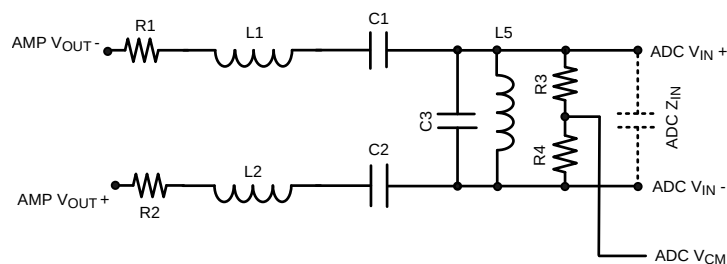
Figure 57. Sample Filter
