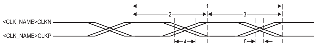
Figure 7-20 Main PLL Transition Time
