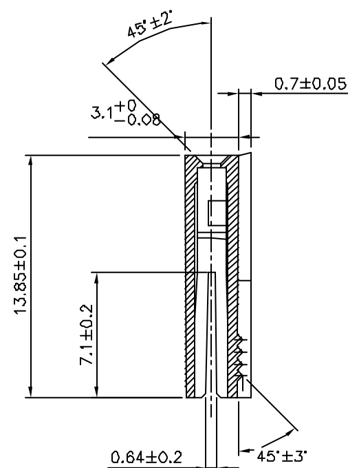
SECTION WW
