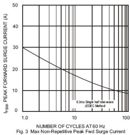
Fig. 3 Max Non-Repetitive Peak Fwd Surge Current
