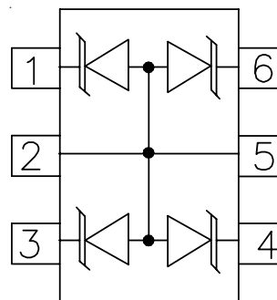
SC-89 (Top View)
