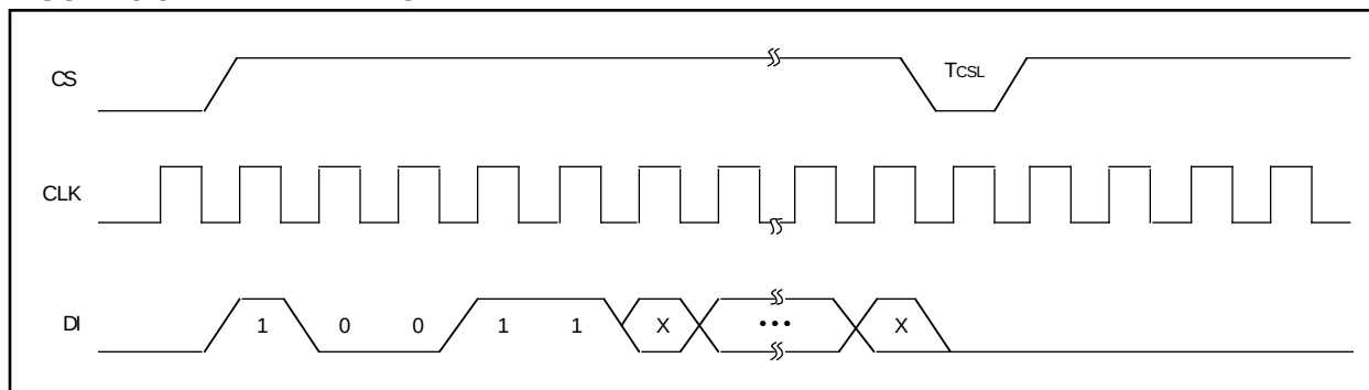
FIGURE 9-3: EWEN TIMING
