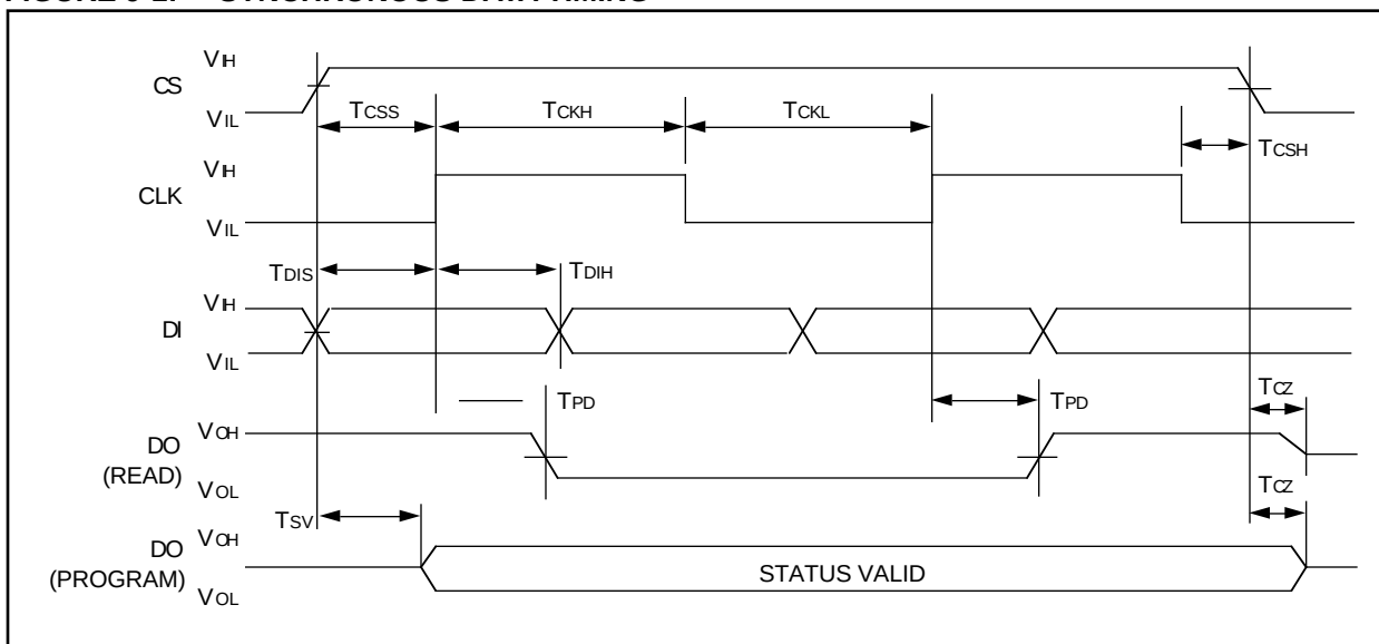
FIGURE 9-2: READ TIMING
