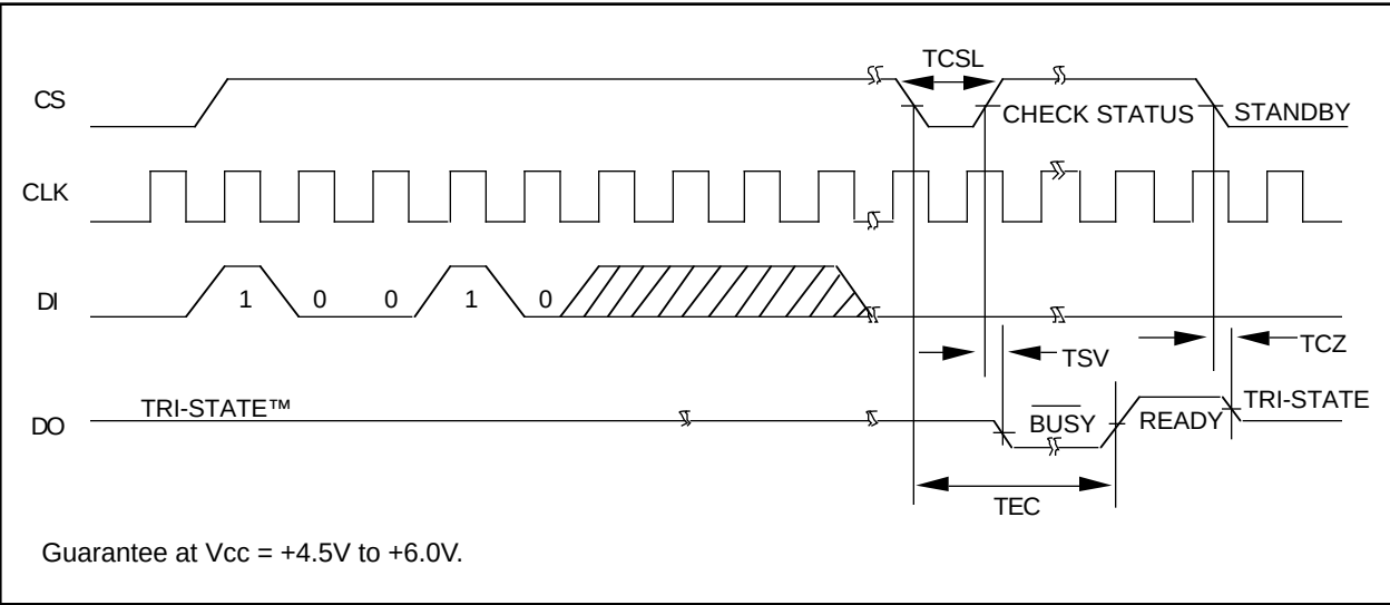
FIGURE 9-8: ERAL TIMING
