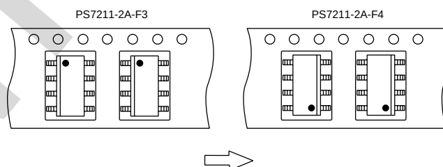
TAPE DIRECTION
