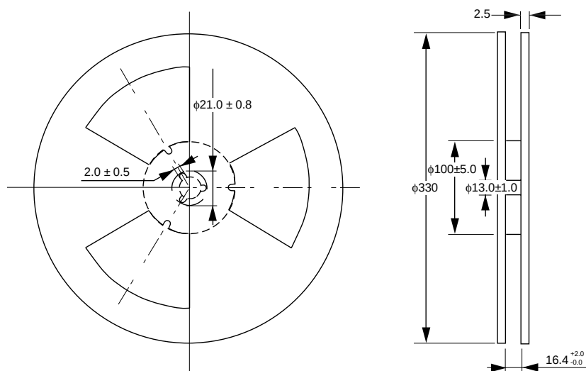
REEL OUTLINE and DIMENSIONS
