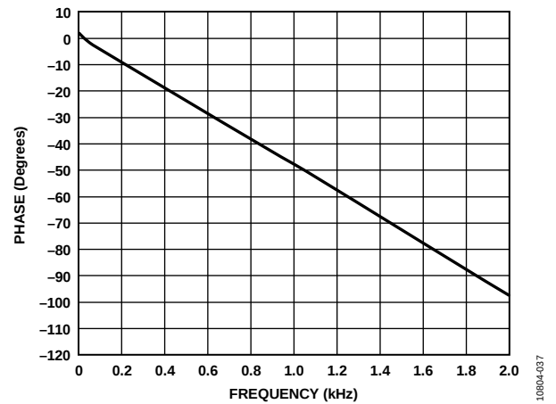
Figure 38. Phase vs. Frequency, 2 kHz Bandwidth, f_s = 48 kHz, Signal Path = DAC_SDData to ASRC to LOUtlx
