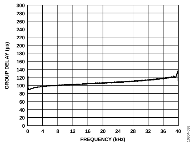
Figure 39. Group Delay vs. Frequency, f_s = 96 kHz, Signal Path = DAC_SDData to ASRC to LOUtlx
