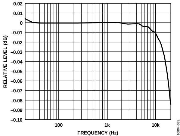
Figure 34. Relative Level vs. Frequency, f_s = 48 kHz, Signal Path = DAC_SDData to ASRC to LOUtlx
