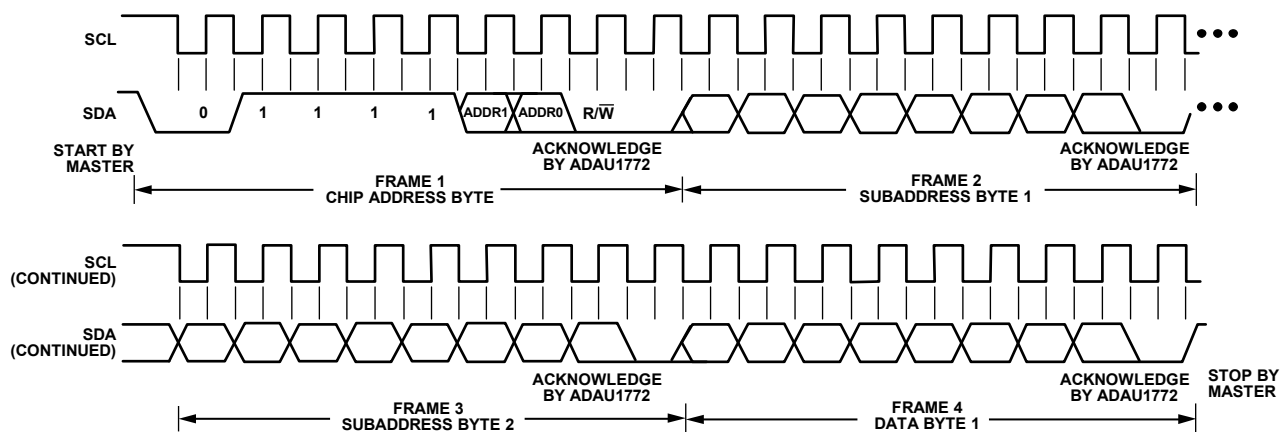
Figure 83. I 2 C Write to ADAU1772 Clocking
