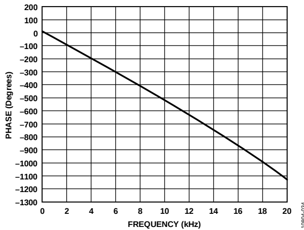
Figure 35. Phase vs. Frequency, 20 kHz Bandwidth, f_s = 48 kHz, Signal Path = DAC_SDData to ASRC to LOUtlx
