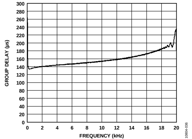
Figure 37. Group Delay vs. Frequency, f_s = 48 kHz, Signal Path = DAC_SDData to ASRC to LOUtlx
