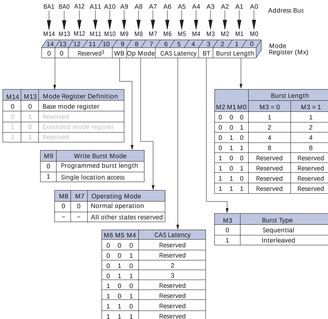
Figure 6: Mode Register Definition
