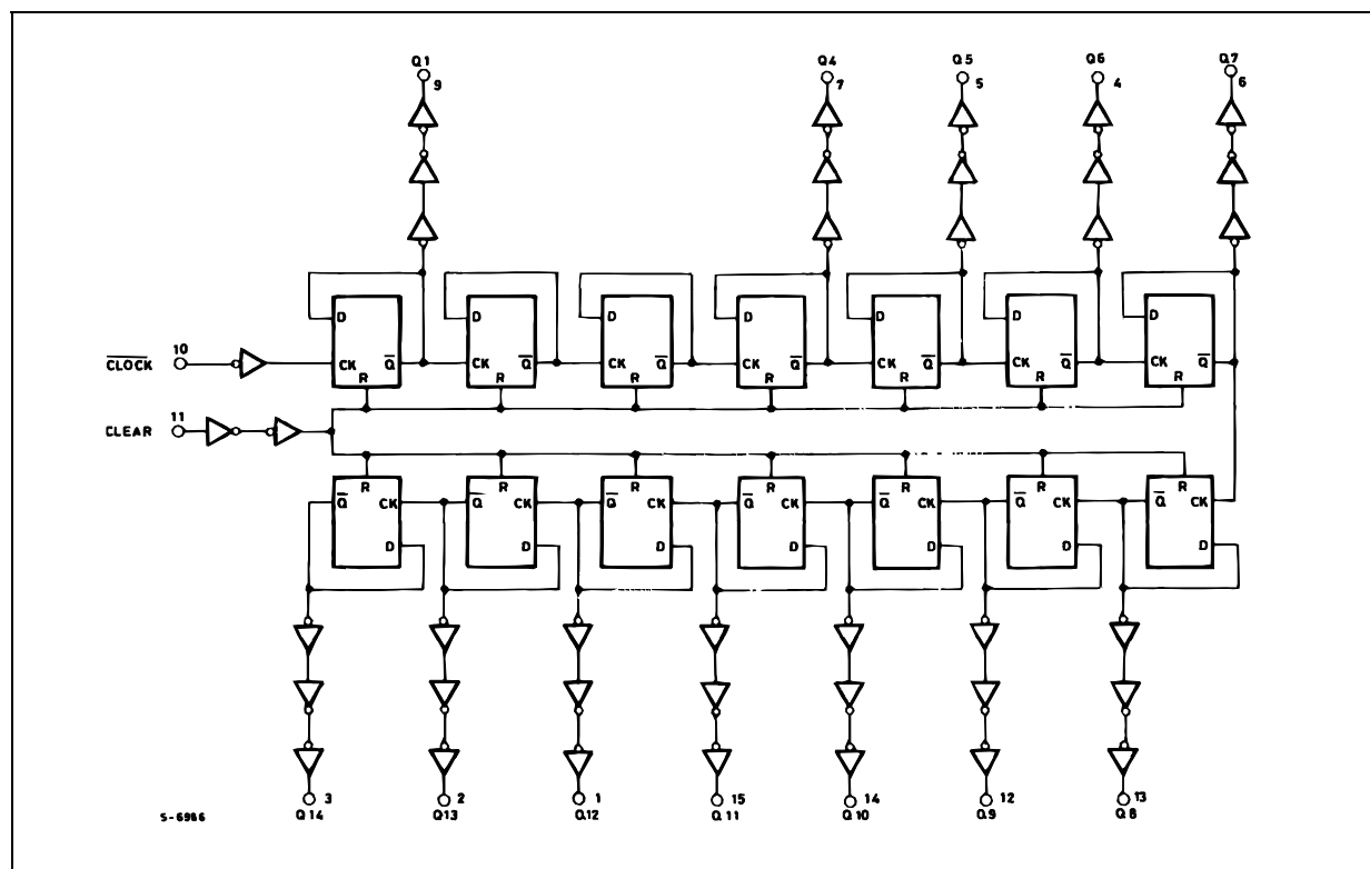
Figure 3: Logic Diagram
