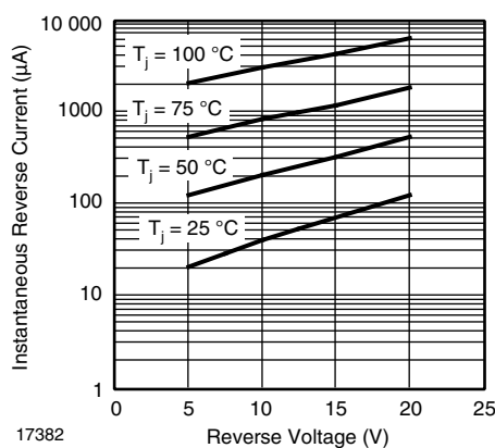
Fig. 4 - Typical Reverse Current Characteristics - SL02
