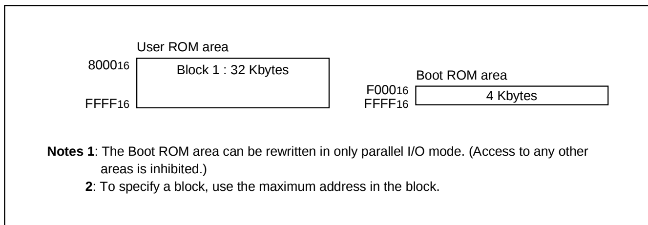
Fig. 116 Block diagram of built-in flash memory
