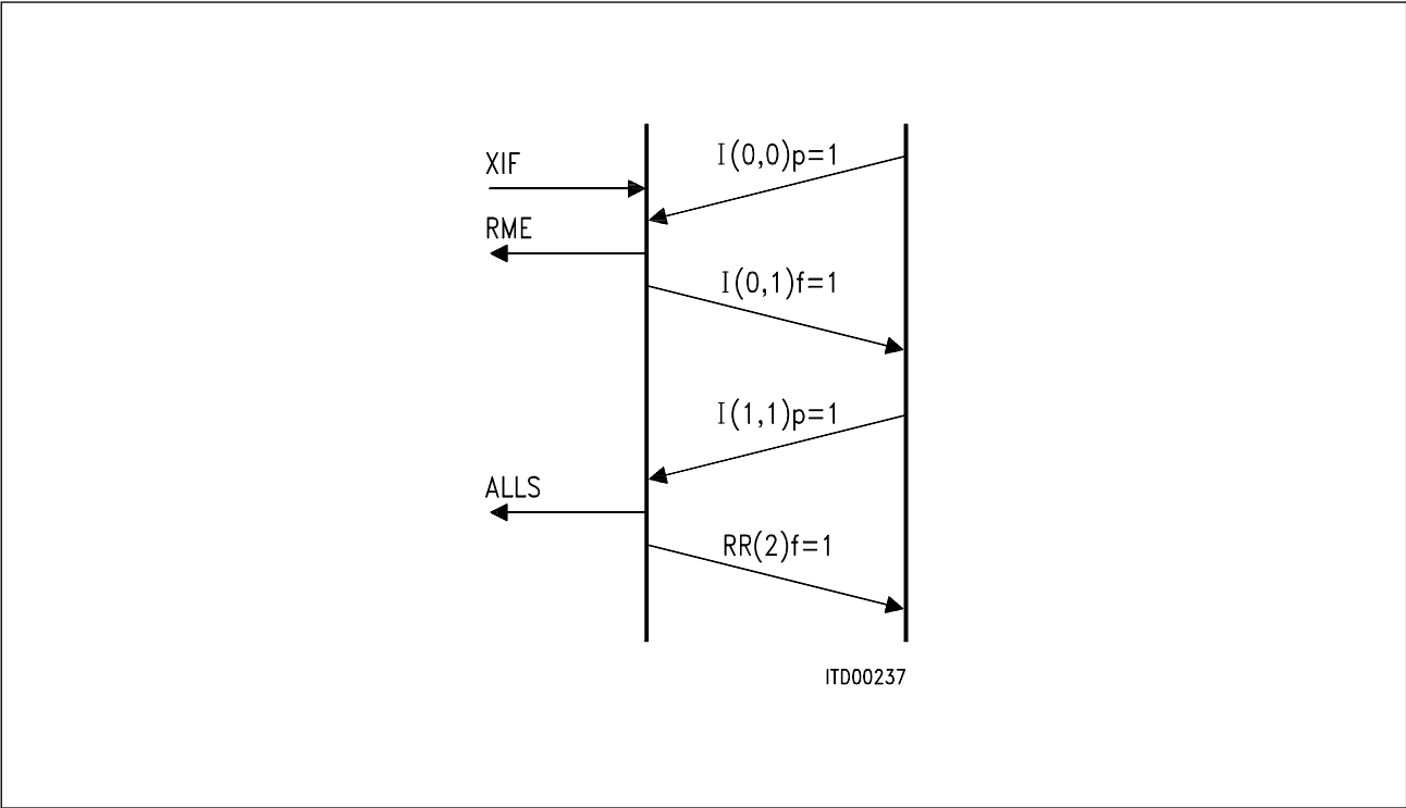
Figure 28 Data Reception/Transmission
