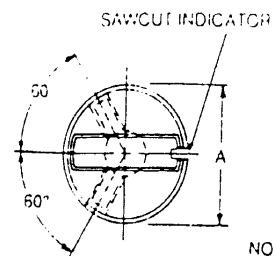
CONTROL KNOB WITH SAWCUT INDICATOR
